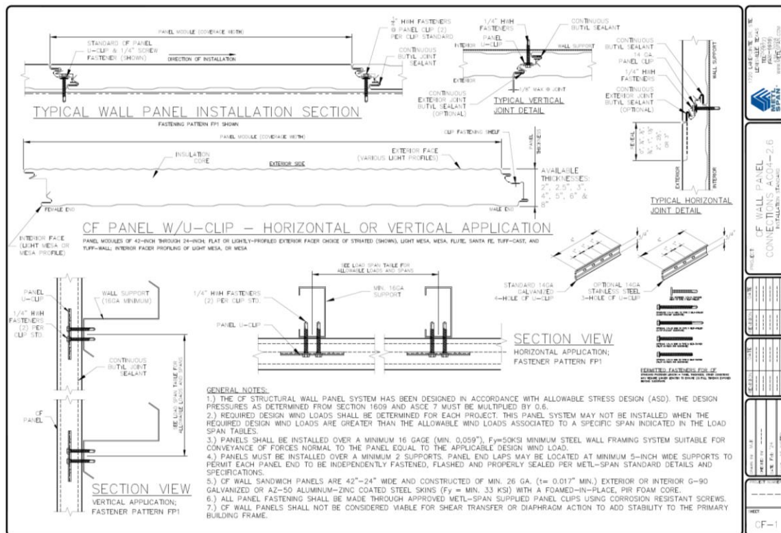
Figure 2: Installation of CF Wall Panels using U-Clips
