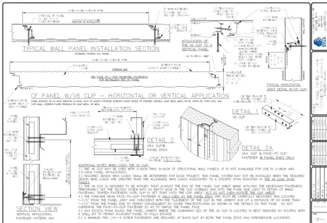
Figure 3: Installation of CF Wall Panels using V6 Clips
